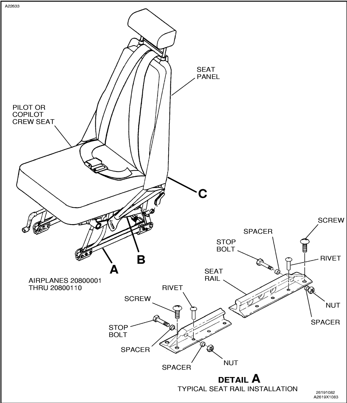
Figure 201 : Sheet 1 : Crew Seat Installation
